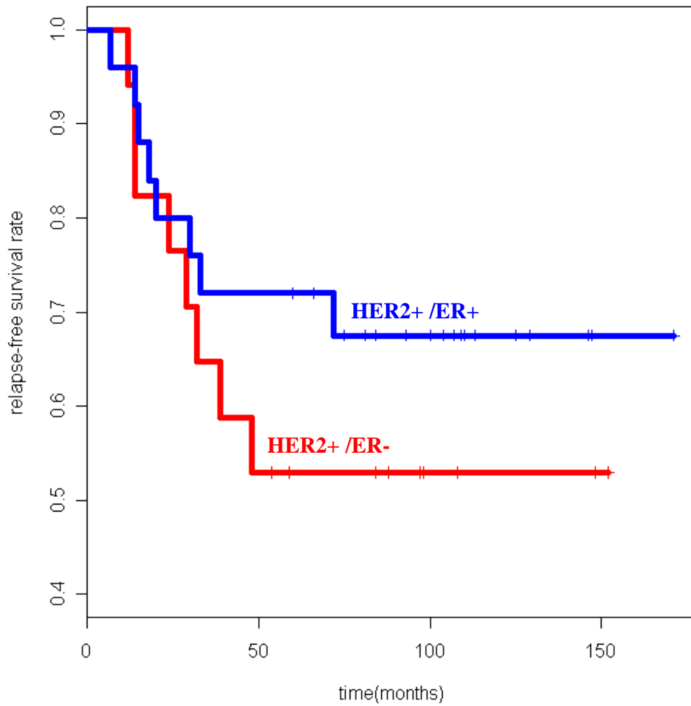
Figure A6-2. Kaplan-Meier relapse free survival curves if the HER2+ subtype is split by ER status. The log-rank p value for the difference in survival between HER2+/ER+ and HER2+/ER- is p = 0.34 , which is not statistically significant.
