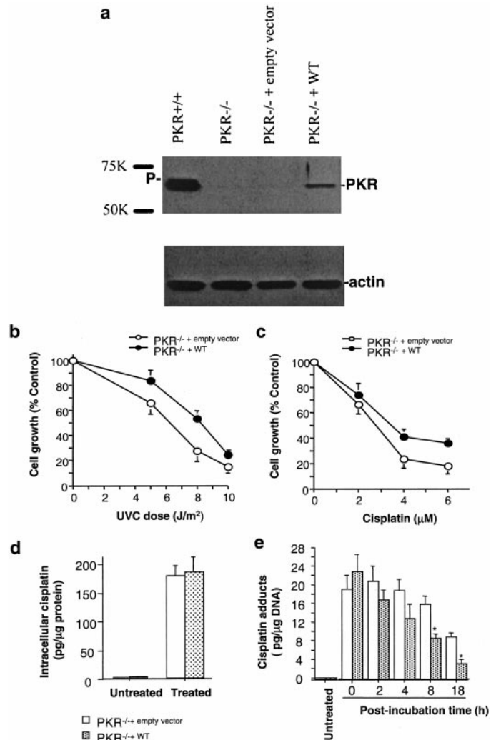
Fig. 4. Effect of PKR expression on drug resistance and cisplatin adduct removal. a, PKR^{-/-} cells transduced with wild-type murine PKR ( PKR^{-/-} + WT ) showed lower expression when compared with the endogenous protein level of mouse ( PKR^{+/+} ) cells. Upper band, hyperphosphorylated form of PKR. The blot was stripped and re-probed with anti-actin (Boehringer Mannheim). Restoration of WT PKR confers resistance to cisplatin (b) and UV (c) as measured by live cell counting. PKR^{-/-} + WT and PKR^{-/-} + empty\ vector do not differ in cisplatin uptake or adduct formation (d), but PKR^{-/-} + WT have demonstrated enhanced adduct removal kinetics relative to PKR^{-/-} + empty\ vector (e). Bars: b–e, SEM.
