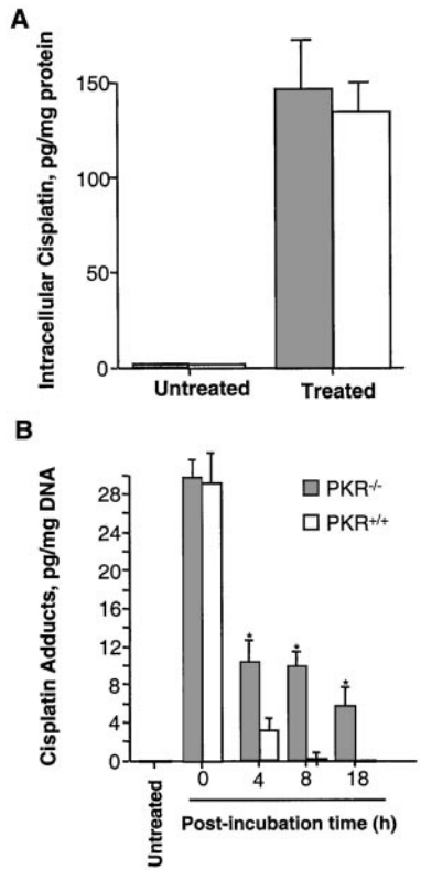
Fig. 3. Cisplatin uptake and DNA adduct formation and removal in PKR^{+/+} and PKR^{-/-} cells. Cells were treated with 25 \mu M cisplatin for 3 h and postincubated with drug-free medium for the indicated times. Cisplatin uptake (a) and adduct formation and removal (b) were measured by atomic spectrometry as described in "Materials and Methods." Bars, SEM for two independent experiments, each performed in duplicate. *, significantly different from PKR^{+/+} at P < 0.001 .
