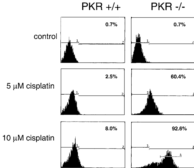
Fig. 2. Cisplatin-induced apoptosis in PKR^{+/+} and PKR^{-/-} cells. PKR^{-/-} cells are susceptible to cisplatin-induced apoptosis. Cells were harvested after 48 h of exposure to 5 or 10 \mu M cisplatin and then analyzed by fluorescence-activated cell sorter after terminal DNA labeling (TUNEL). The percentage of apoptotic cells is indicated.
