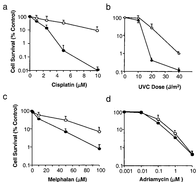
Fig. 1. Cytotoxic effect of DNA-damaging agents on PKR^{+/+} and PKR^{-/-} cells. PKR^{+/+} (○) and PKR^{-/-} (●) cells were exposed to cisplatin, melphalan, or Adriamycin for 96 h or to UVC, and then cytotoxicity was assayed by MTT. PKR^{-/-} cells were significantly more sensitive to bulky adduct-inducing agents (a–c) than PKR^{+/+} cells but showed no increase in sensitivity to Adriamycin (which induces double strand breaks; d). Bars, SEM.
