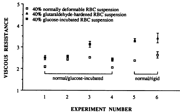
Fig. 3. Intratumor viscous resistance in 4 trials (experiments 1 through 4) of alternate perfusion with normally deformable (□) and glucose-incubated (■) RBC suspensions and in 2 trials (experiments 5 and 6) with normally deformable and glutaraldehyde-hardened (▲) RBC suspensions at 40% hematocrit. Bars, propagation of the standard deviation associated with the least squares fit of the linear pressure-flow curve.
