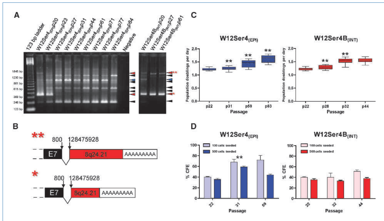
Figure 2. Retention of HPV16 episome-derived transcripts and acquisition of a growth advantage in W12Ser4 (EPI) (left) and W12Ser4B (INT) (right). A, APOT analysis of W12Ser4 (EPI) (left) and W12Ser4B (INT) (right). Blue arrows, expected size of episome-derived transcripts (1,050 bp); black arrows, nonspecific products; red arrows, integrant-derived transcripts. The far left and right lanes of the left panel show DNA molecular weight markers and a no-template negative control, respectively. As the panels represent two independent APOT assays, there are differences in band intensities and background signal in the two samples at the point of divergence of W12Ser4 (EPI) and W12Ser4 (INT) (passage 20; lane 2 in left panel; lane 1 in right panel). B, schematics of the low molecular weight (*) and high molecular weight (**) integrant-derived transcripts detected throughout long-term culture in W12Ser4B (INT) and at early passages in W12Ser4 (EPI) . Viral and host sequences are shaded black and red, respectively. Numbers above each schematic indicate the genomic positions of the viral and host sequence at the splice junction. C, growth rate of W12Ser4 (EPI) and W12Ser4B (INT) , expressed as population doublings per day. Boxes show the median growth rate and interquartile range, and whiskers represent the maximum and minimum values. D, CFE of W12Ser4 (EPI) and W12Ser4B (INT) , calculated after seeding either 100 or 500 cells. Columns, mean of three independent platings; bars, SE. In both C and D, asterisks (**) indicate a significantly different growth rate/CFE compared with the previous passage analyzed ( P < 0.05 , two-sample t test).
