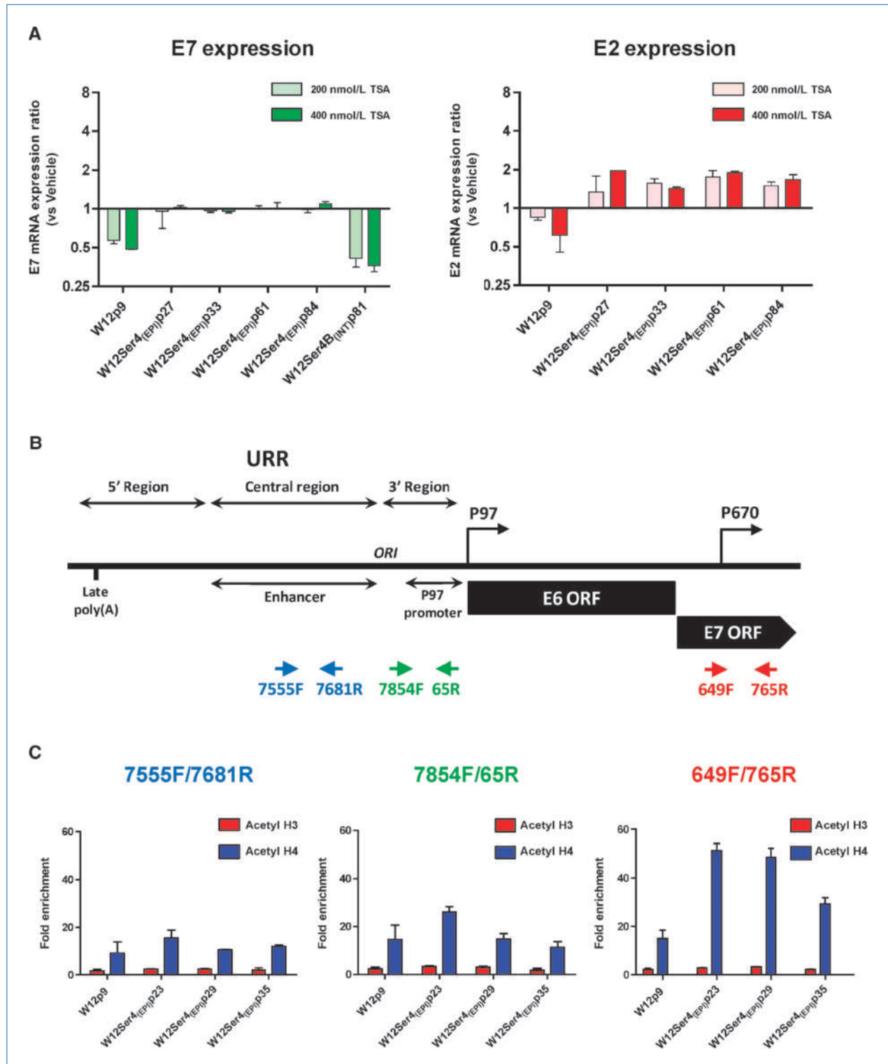
Figure 6. Analysis of changes in histone acetylation state around the HPV16 URR in W12Ser4 EPI . A , qPCR analysis of E7 and E2 mRNA expression (versus vehicle-only controls) following treatment of cells with TSA at either 200 or 400 nmol/L for 2 h. B , schematic of the HPV16 URR, early promoter (P97), and late promoter (P670) regions. Arrowheads in blue, green, and red indicate viral sequences quantified by qPCR following ChIP. C , qPCR analysis of ChIP assays for binding of acetylated histone H3 and H4 around the HPV16 URR. For each cell population analyzed, graphs show FE (versus preimmune serum negative control samples) for sequences at the enhancer (7555F/7681R), early promoter (7854F/65R), or late promoter (649F/765R) following ChIP with antibodies against either acetylated histone H3 or acetylated histone H4.
