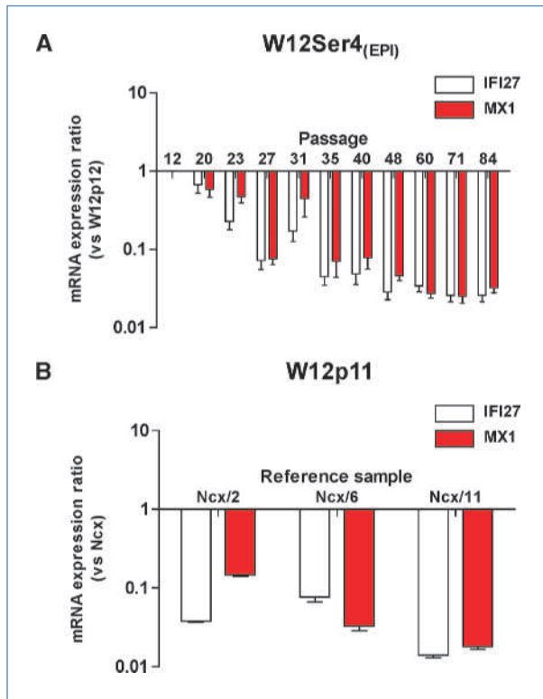
Figure 5. Expression of ISGs in W12Ser4 (EPI) . A and B, qPCR analysis of IFI27 and MX1 mRNA expression in W12Ser4 (EPI) relative to parental W12p12 (A) and in parental W12p11 relative to three normal ectocervical keratinocyte (Ncx) primary cultures (B).
