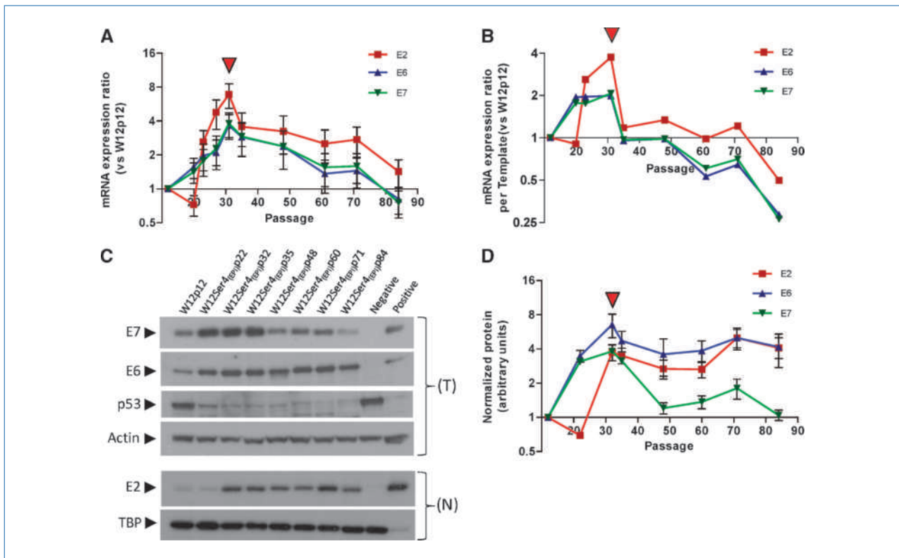
Figure 4. Levels of HPV16 early gene mRNA and protein in W12Ser4 (EPI) . A and B, relative HPV16 early gene mRNA expression in W12Ser4 (EPI) , showing levels overall (A) and per viral copy, calculated using the following formula: mean relative mRNA expression ratio/mean relative HPV16 copy number (B). C, Western analysis of p53 and the HPV16 E6, E7, and E2 proteins. \beta -Actin and TBP represent loading controls for total (T) and nuclear (N) protein extracts, respectively. For detection of E6/E7 protein, controls were total protein from Ncx/2 (negative) and W12Ser2p25 (positive). Because the p53 blot was generated by reprobing the E6 blot, the negative and positive lanes are reversed. For detection of E2 protein, controls were HeLa nuclear protein (negative) and full-length E2 purified from Sf21 insect cells (positive; a kind gift from Norman Maitland). D, viral protein quantification (arbitrary units) by densitometry. Points, mean of technical replicate experiments; bars, SE. In A, B, and D, the red arrowheads indicate the point at which invasiveness was acquired.
